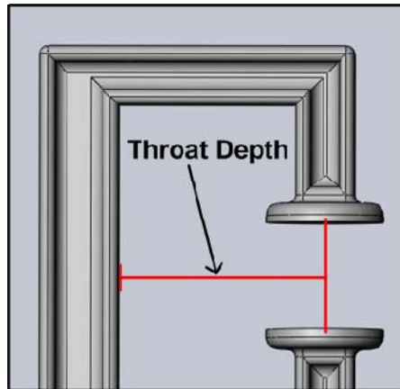
Figure 11: Throat Depth- Each different size and style of clamp has a different throat depth. The throat depth is the distance from the pads of the clamp to the back of the clamp.
